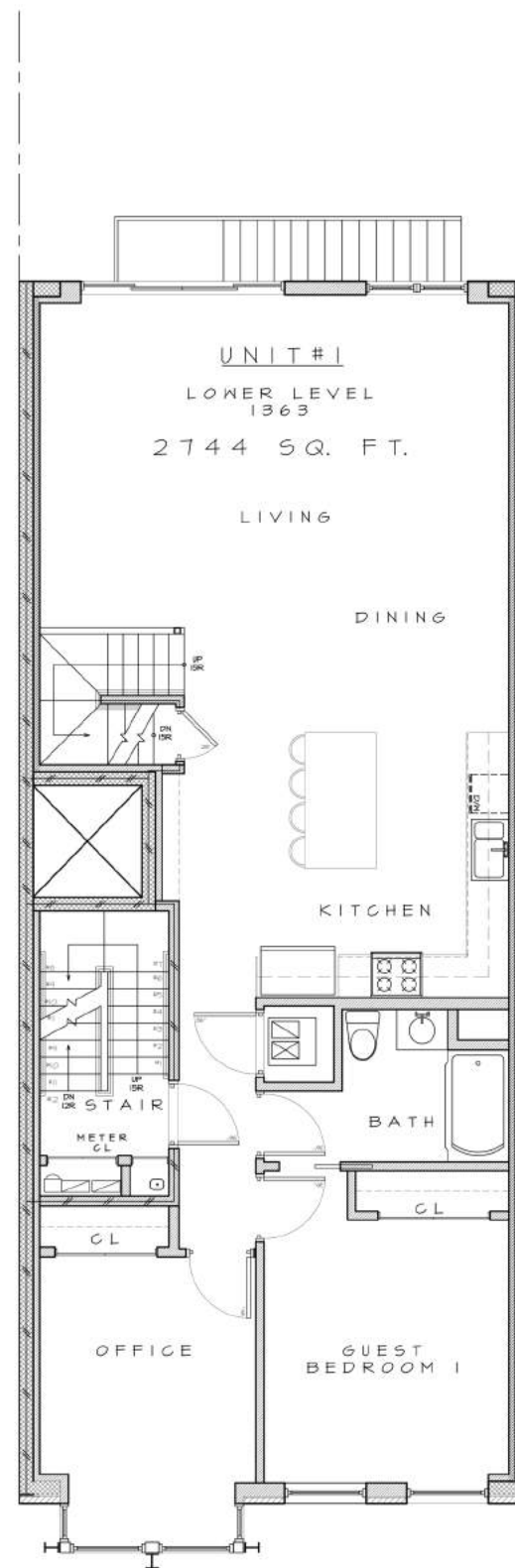
UNIT 1 2ND FLOOR 1363 SQ. FT.
